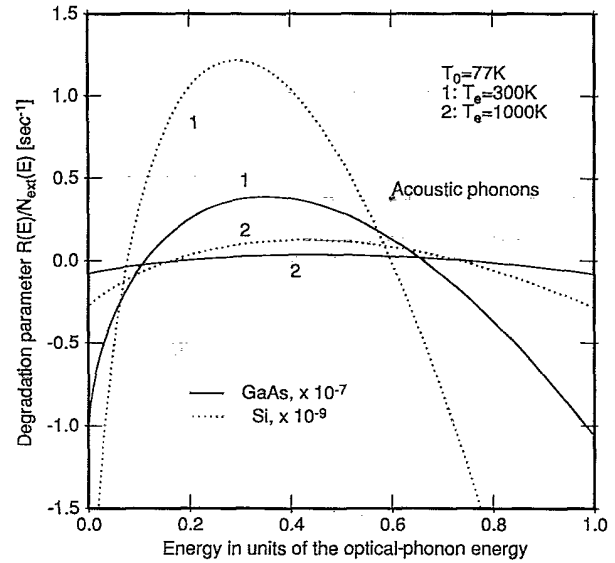
FIG. 2. Degradation parameter R^{\text{ac}}(E)/N_{\text{ext}}(E) calculated according to Eqs. (14) and (15) for the nonequilibrium electron distribution described by Eq. (12) with T_e = 300 and 1000 K and the lattice temperature T = 77 K.
