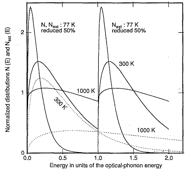
FIG. 1. Normalized distributions N_{\text{ext}}(E) , defined by Eq. (3), and N(E) \propto \sqrt{E} f(E) . Solid lines show N_{\text{ext}} , calculated from Eq. (14); dotted lines correspond to N .
