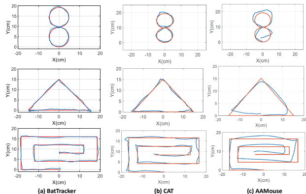
Figure 17: Shapes created by BatTracker, CAT, and AAMouse.
