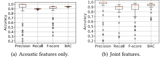
Figure 11: The precision, recall, F-score and BAC of one-class SVM model using acoustic and joint features.
