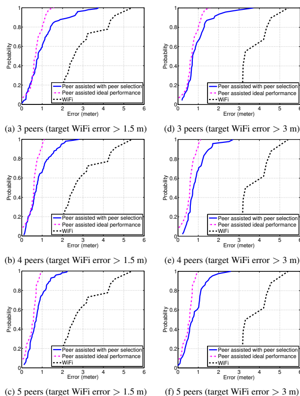
Figure 9: Peer-Assisted localization performance for target phone under different number of peers for HTC EVO. The first column is results when the target WiFi error is greater than 1.5m and the second column with target WiFi error greater than 3m.
