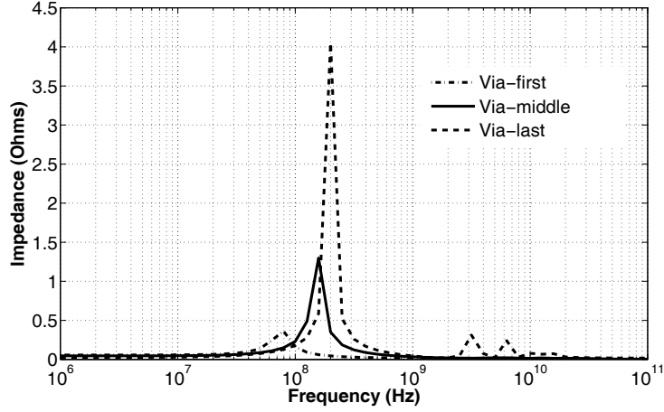
Figure 4.11: Impedance characteristics at the design points listed in Table 4.1 when decoupling capacitance is implemented as MOS capacitors.
