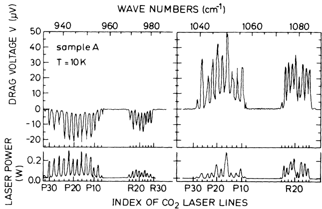
FIG. 3. Low-temperature photon-drag voltage (upper traces) and corresponding laser power (lower traces) for a wide spectrum of CO 2 laser lines. Increasing the photon energy from below to above the intersubband energy of 1027 \text{cm}^{-1} [see Fig. 1(a)] changes the sign of the induced drag voltage from negative to positive.
