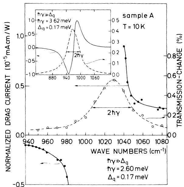
FIG. 4. Experimental intersubband-resonance transmission change per transversed quantum well from Fig. 1(a) (O) and photon-drag short-circuit current, normalized on the laser-power density and sample length (●), respectively. Lines are guides to the eye. Inset: Calculated spectra from Ref. 11, whose parameters are very close to the experimental ones as indicated in the figure. The axis scales of the inset refer to the lettering of the main figure.
