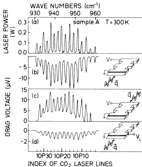
FIG. 2. (a) CO 2 laser power for different lines of the 10P band, representing a quasifrequency sweep. (b)–(d) Room-temperature photon-drag effect voltage vs frequency for \hbar\omega < \hbar\omega_{21} and different experimental setups as indicated on the right-hand-side insets. In reversing \mathbf{q} , the drag voltage is reversed. The transverse photon drag is about 1 order of magnitude smaller [(d)] than the longitudinal [(b) and (c)] one.
